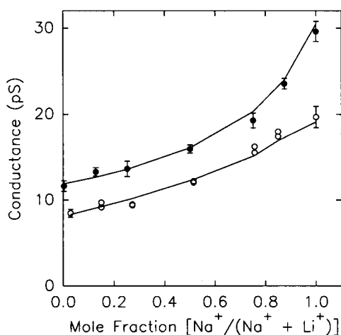
FIGURE 6 Conductance at 0 mV of BTX-modified Na + channels from rat muscle as a function of the activity mole fraction of Na + in Na + -Li + symmetrical mixtures. Open circles, 206 mM total ionic strength; closed circles, 2,006 mM total ionic strength. Solid lines refer to predictions of the 3B2S model with parameters for Na + and Li + in Table 1.
