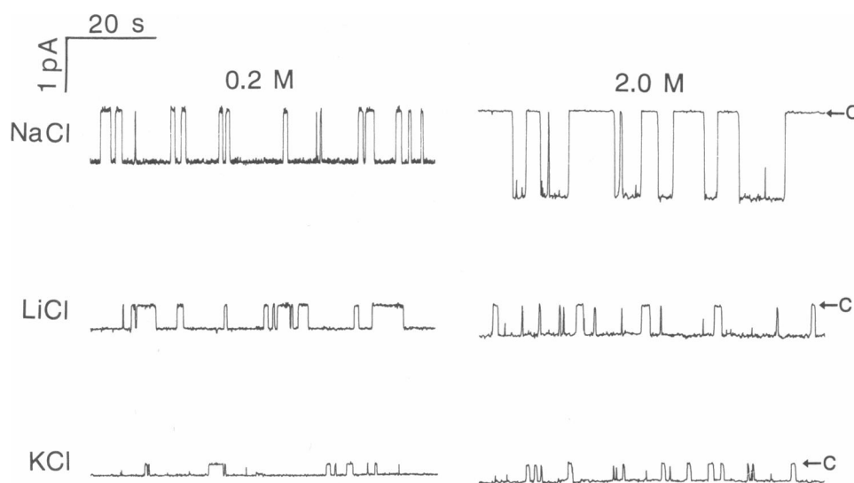
FIGURE 2 Comparison of single-channel currents in the presence of various permeant ions. \text{Na}^+ channel currents were recorded in the presence of symmetrical solutions containing either 0.2 M NaCl, LiCl, or KCl (left) or 2.0 M NaCl, LiCl, or KCl (right). The holding voltage was -50 mV in all cases and openings are downward, as indicated by arrows marking the closed (c) current level. Discrete blocking events are due to the presence of 20 nM (left records) or 200 nM (right records) decarbamoylsaxitoxin on the external side of the channel.
